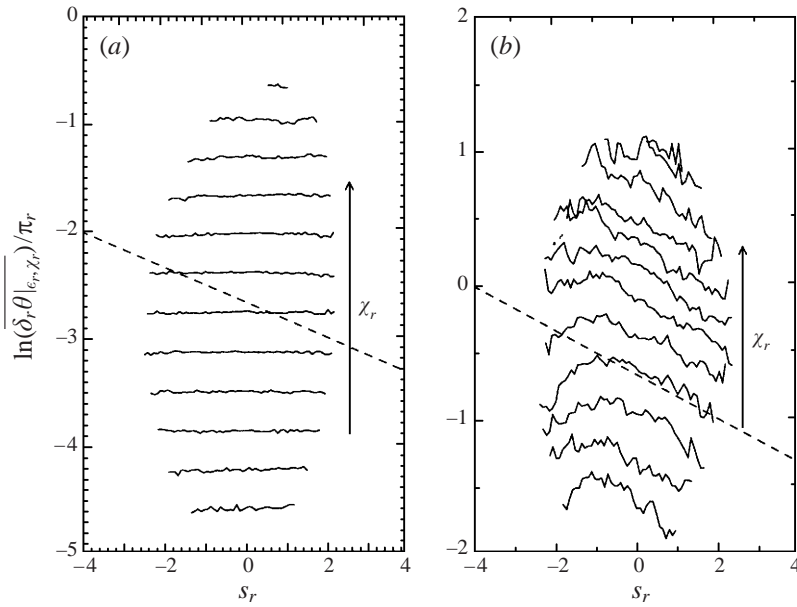
FIGURE 17. Scalar increment conditioned on the locally averaged dissipation rates, \delta_r \theta|_{\epsilon_r, \chi_r} , against s_r on a log-log plot, for the 256^3 forced DNS field f256 at R_\tau = 151 and Pr = 1 . Each curve corresponds to a fixed r and \chi_r . (a) r = \Delta ; (b) r = 50\Delta . The dashed line shows -\frac{1}{6} slope. s_r \equiv (\ln \epsilon_r - m_r)/\sigma_r .
