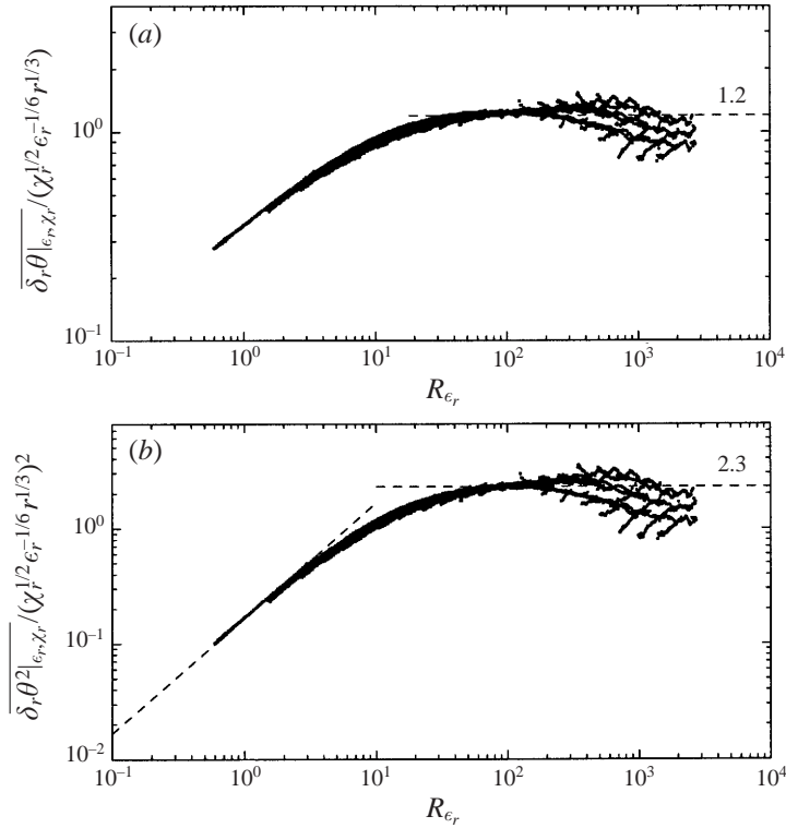
FIGURE 22. As figure 21 but for the 512^3 DNS field at R_\lambda = 195 and Pr = 1 .
